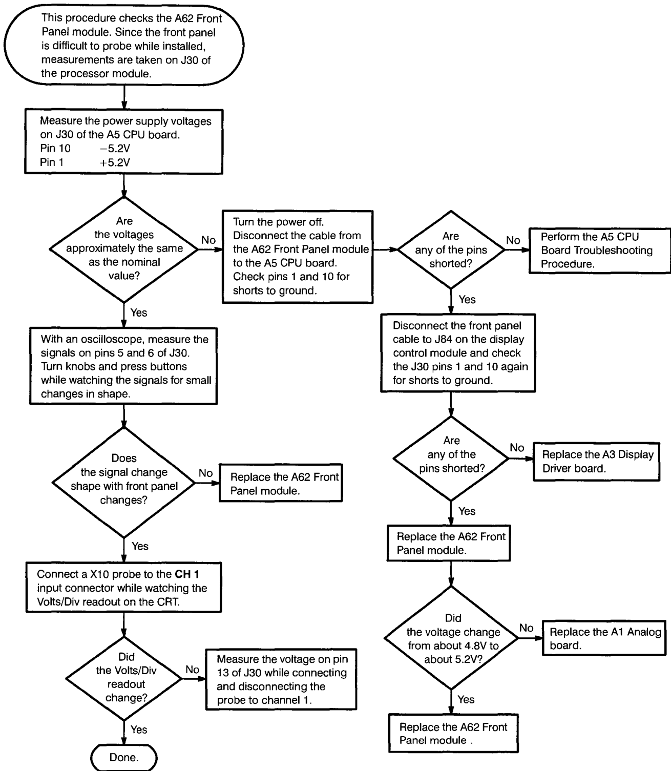
Figure 6-24: A62 Front Panel module Troubleshooting Procedure
