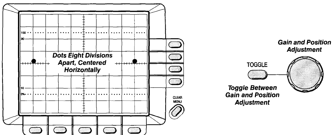
Figure 5-4: Horizontal Adjustments
