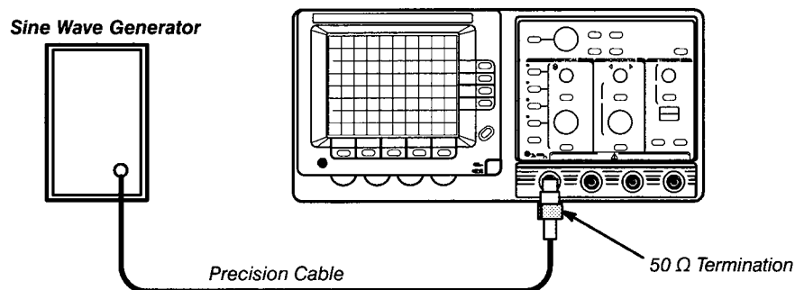
Figure 4-12: Trigger Sensitivity Test Setup One
