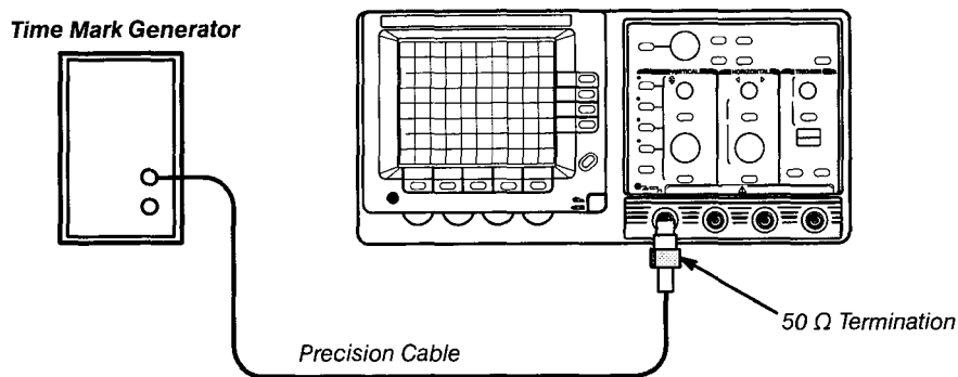
Figure 5-2: CRT Adjustments Calibration Setup
