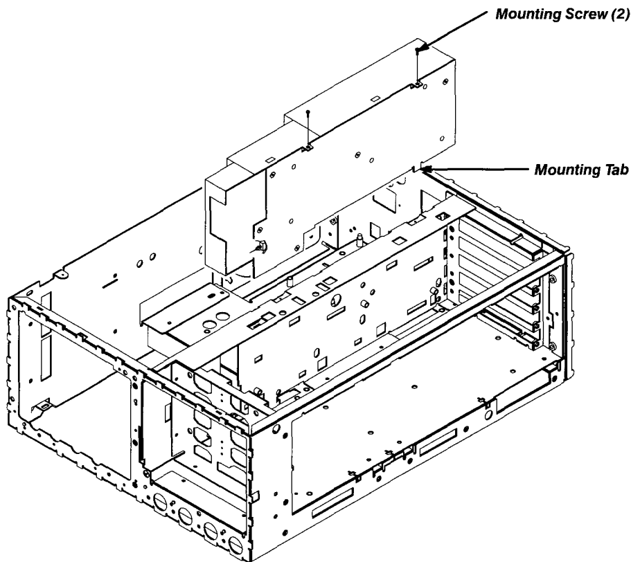
Figure 6-19: Power Supply Removal
