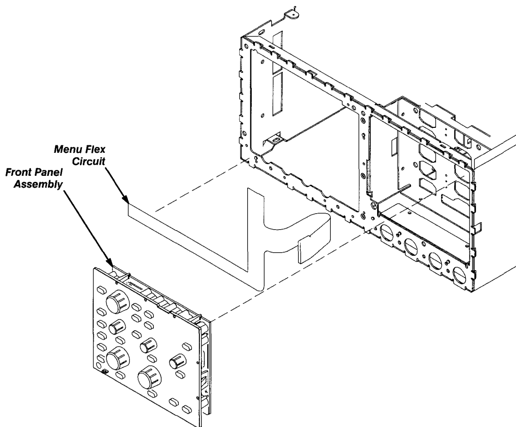
Figure 6-13: Menu Flex Circuit Board Removal
