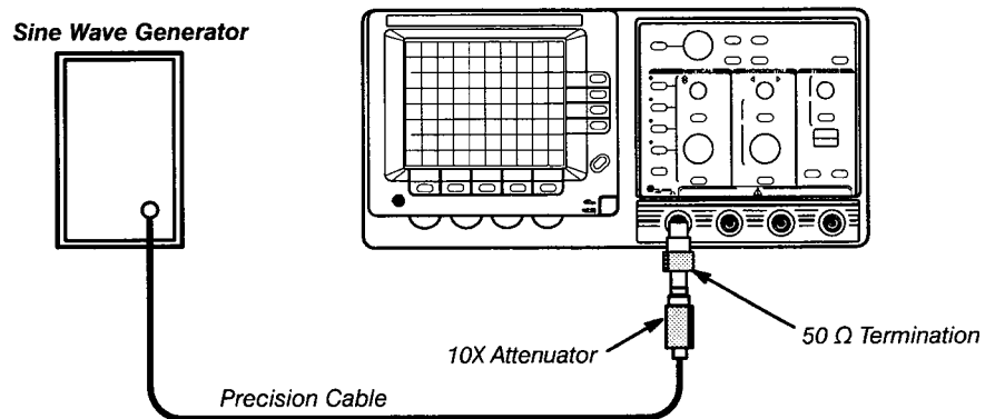
Figure 4-13: Trigger Sensitivity Test Setup Two
