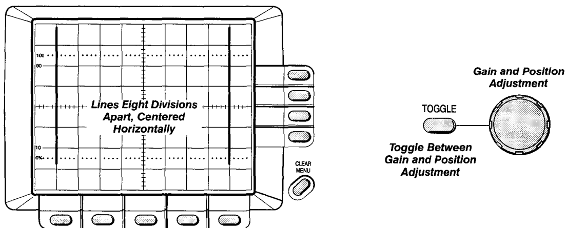
Figure 5-6: Horizontal Adjustments
