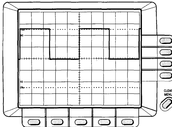
Figure 2-4: Probe Compensation Signal Displayed after AUTASET
