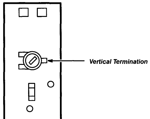
Figure 5-13: TAS 485 Vertical Termination Hybrid Adjustment
