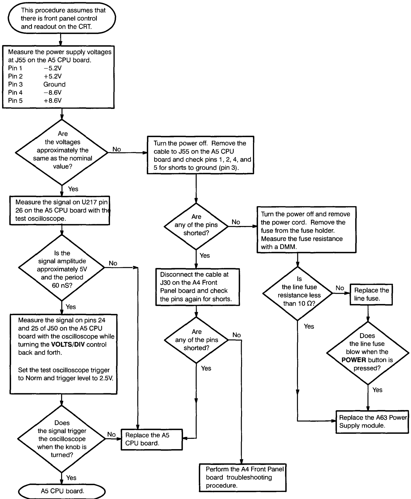
Figure 6-21: A5 CPU Board Troubleshooting Procedure
