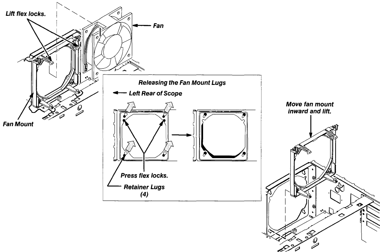
Figure 6-20: Fan and Fan Mount Removal
