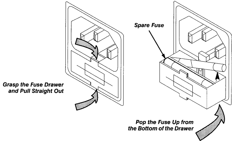
Figure 2-2: Fuse Compartment
