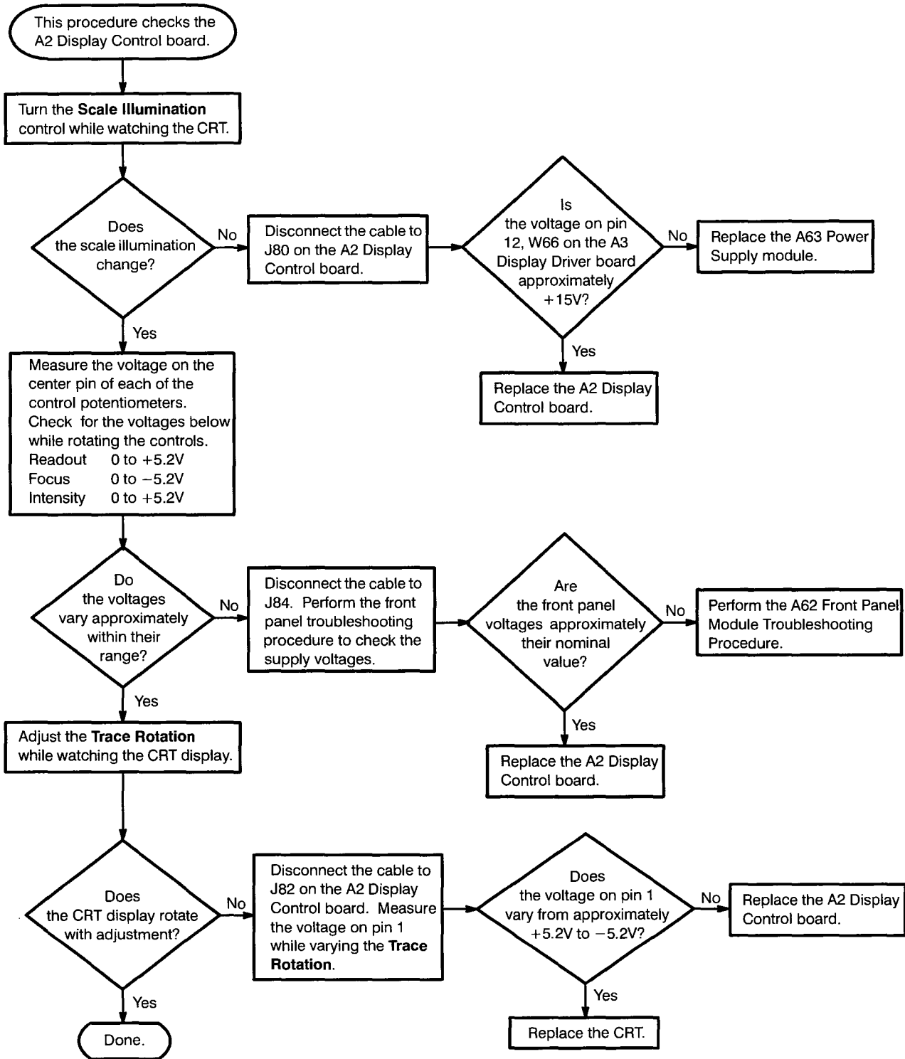
Figure 6-25: A2 Display Control Board Troubleshooting Procedure
