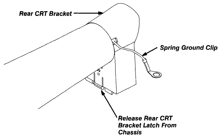
Figure 6-16: CRT Rear Bracket and Ground Clip
