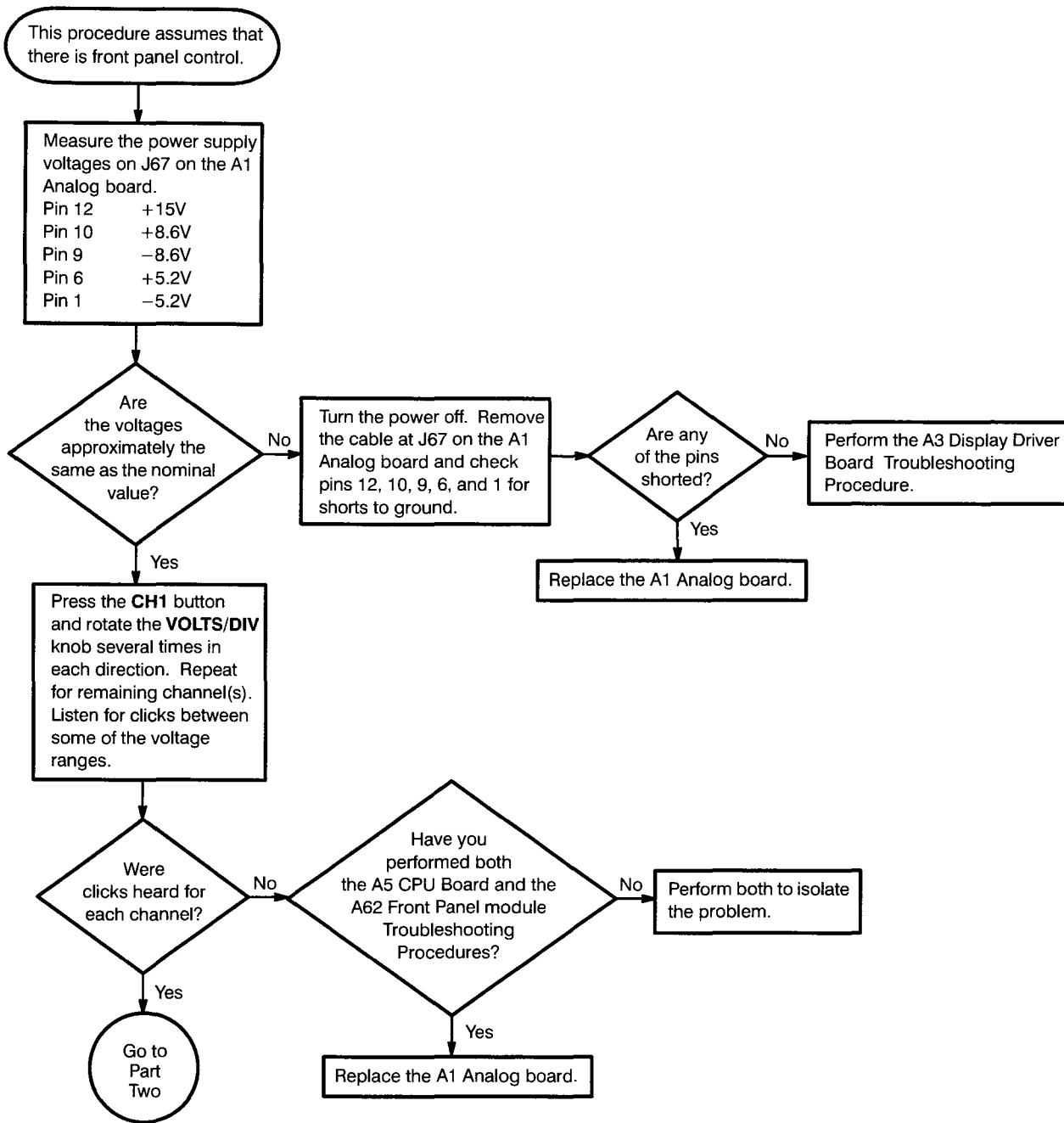
Figure 6-22: A1 Analog Board Troubleshooting Procedure
