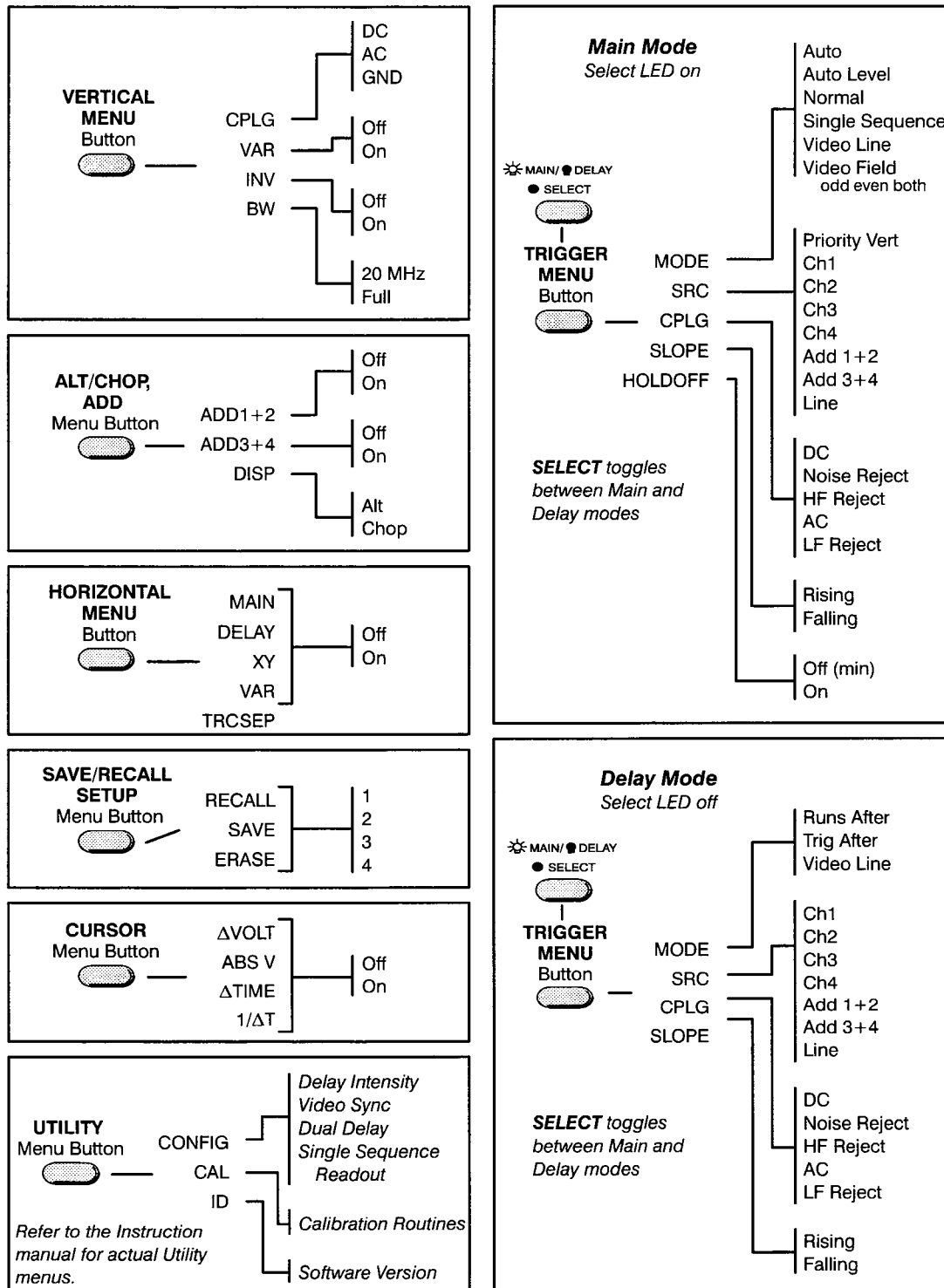
Figure 2-8: Menu Map
