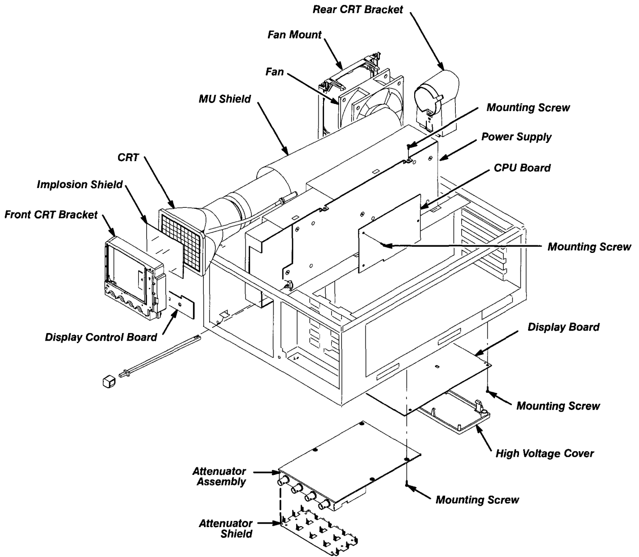
Figure 6-3: Internal Modules
