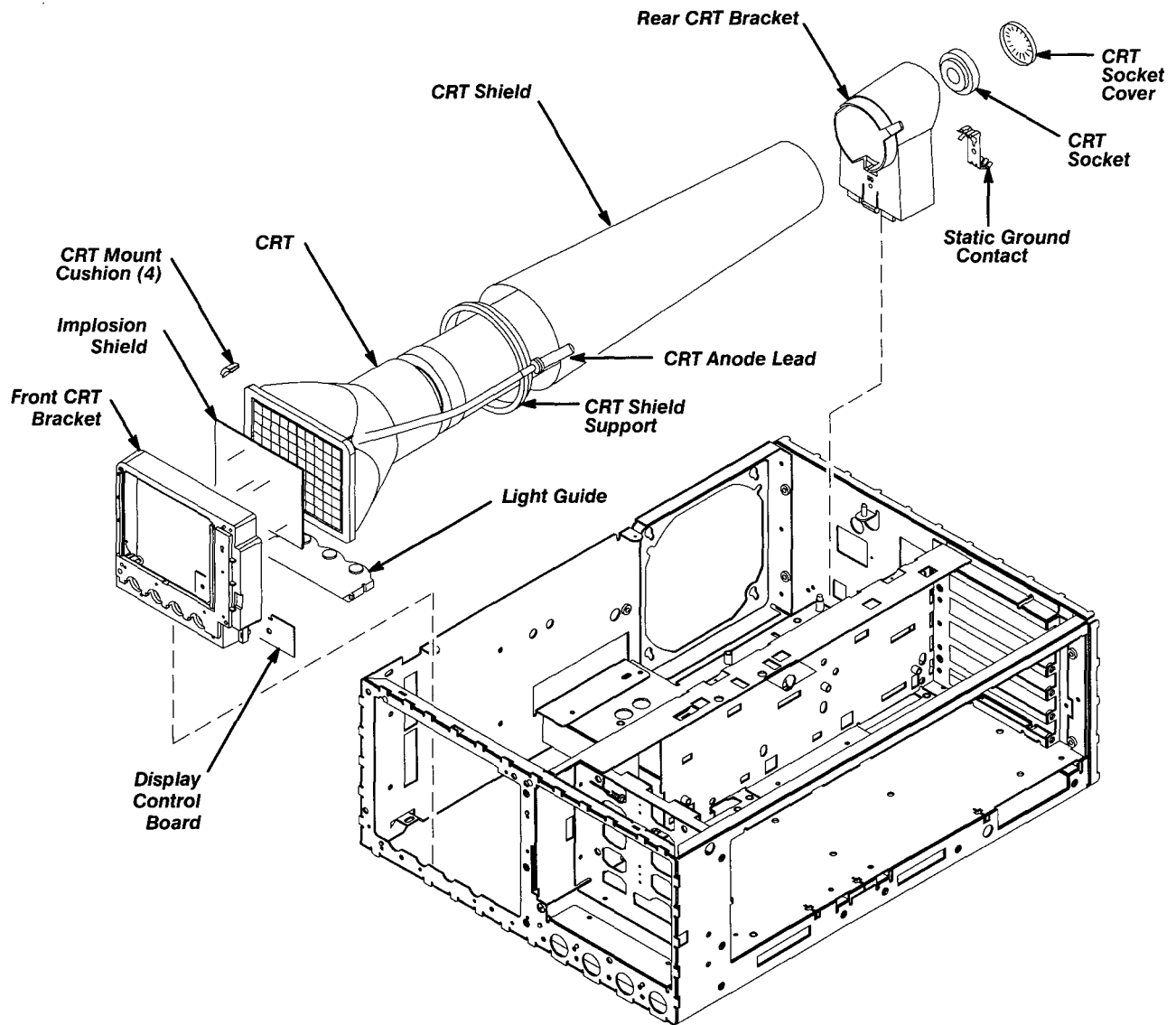
Figure 6-17: CRT Removal
