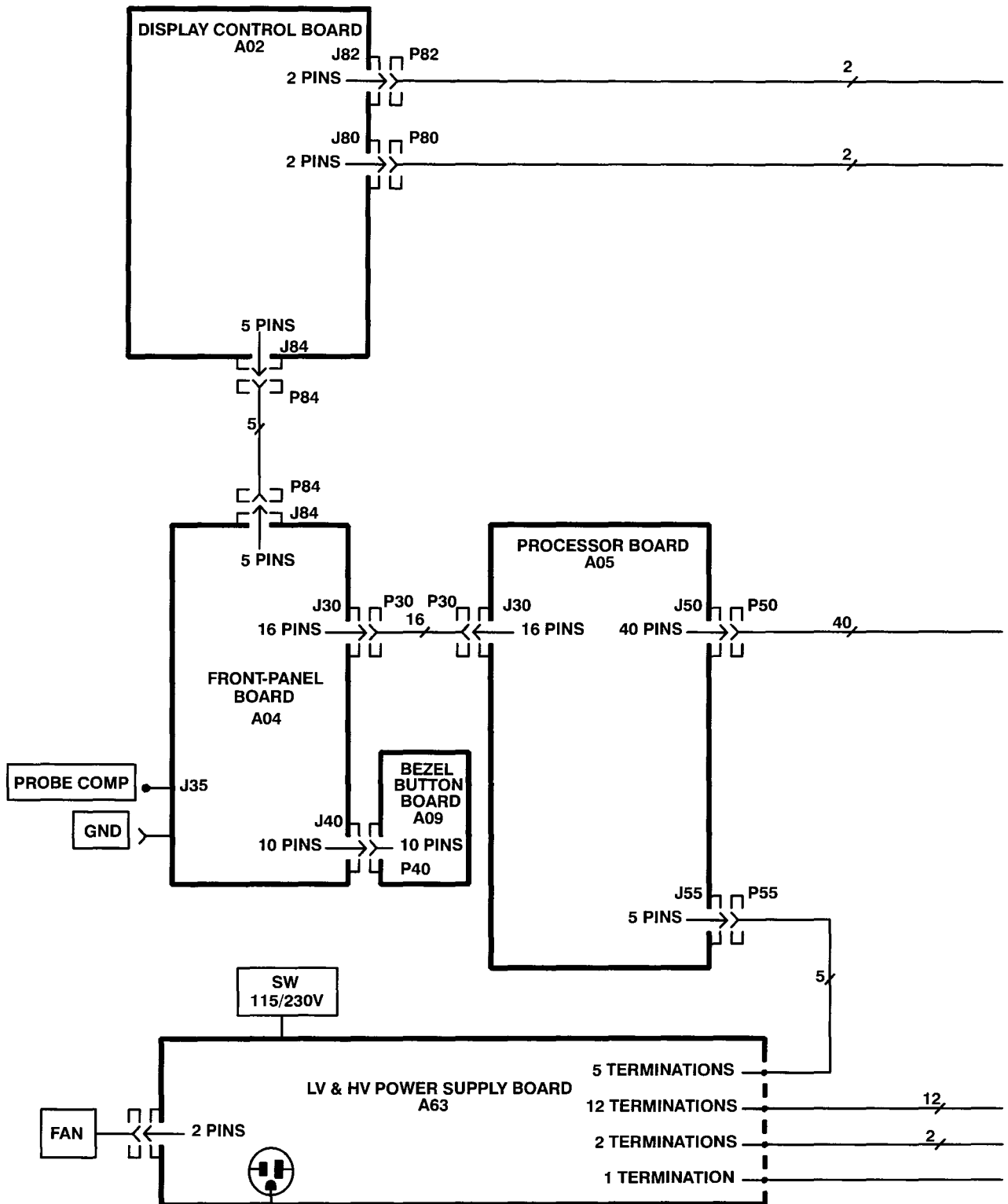
Figure 3-1: Block Diagram
