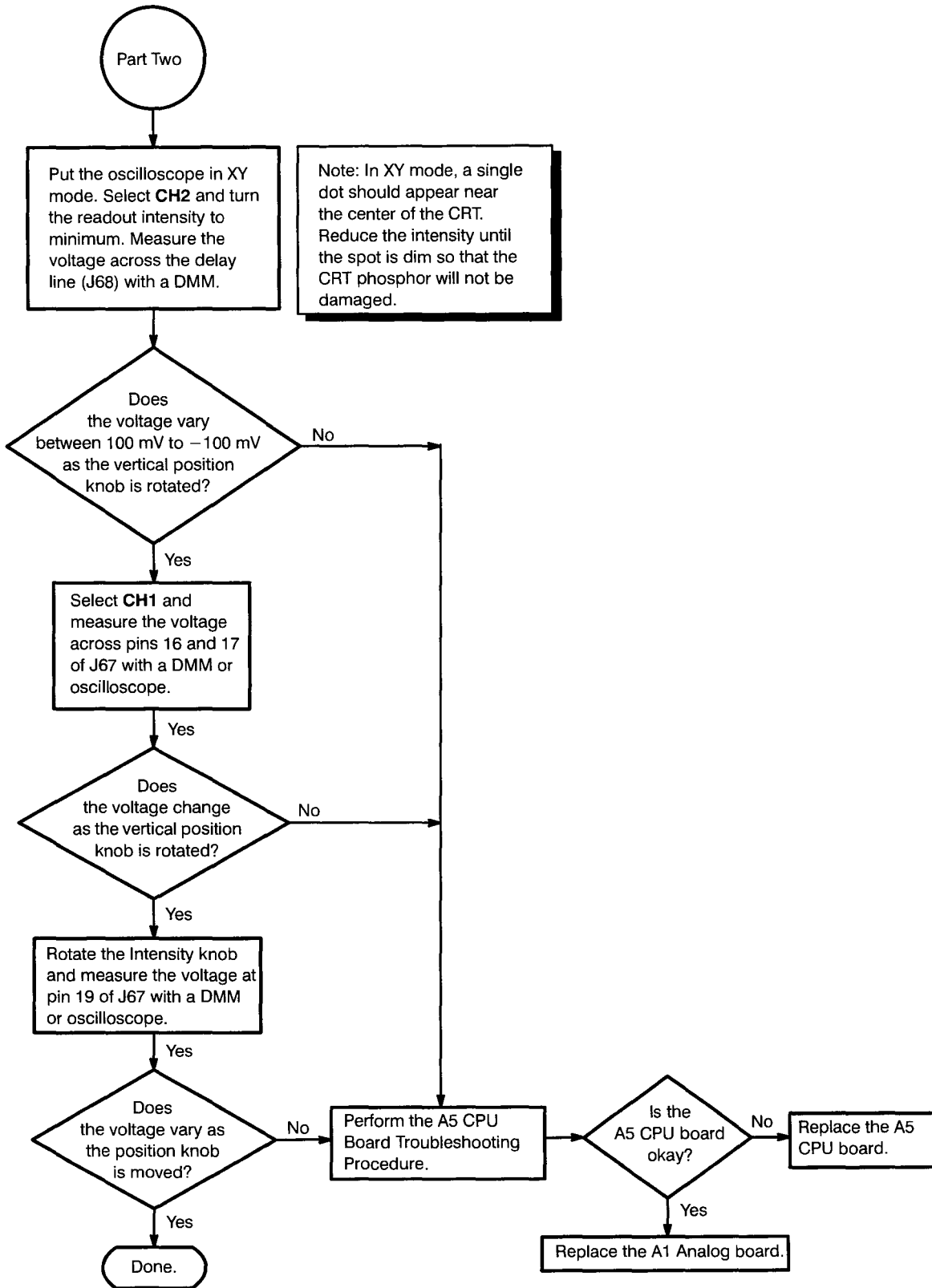
Figure 6-22: A1 Analog Board Troubleshooting Procedure (Cont.)
