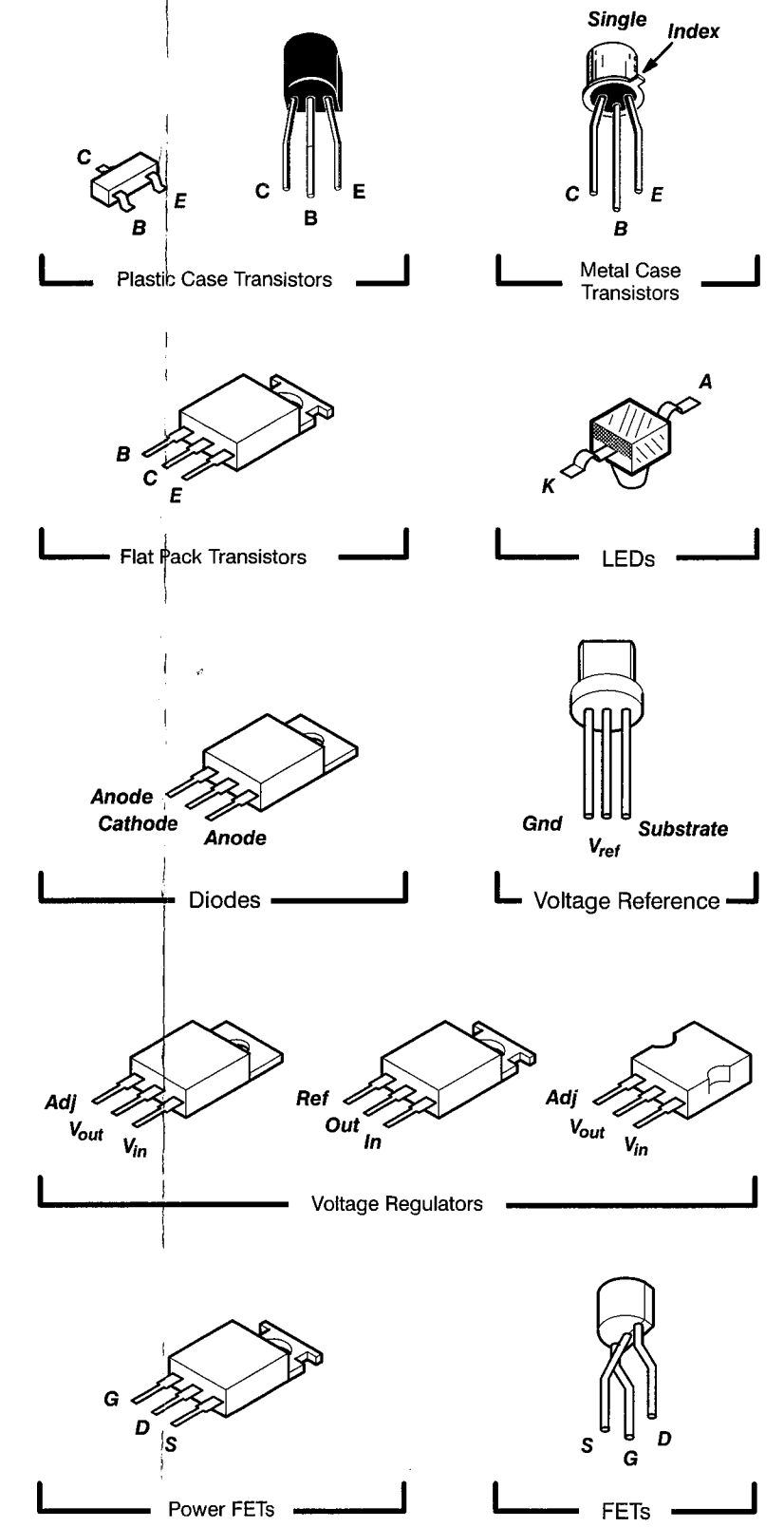
Figure 9-3: Semiconductor Lead Configurations
