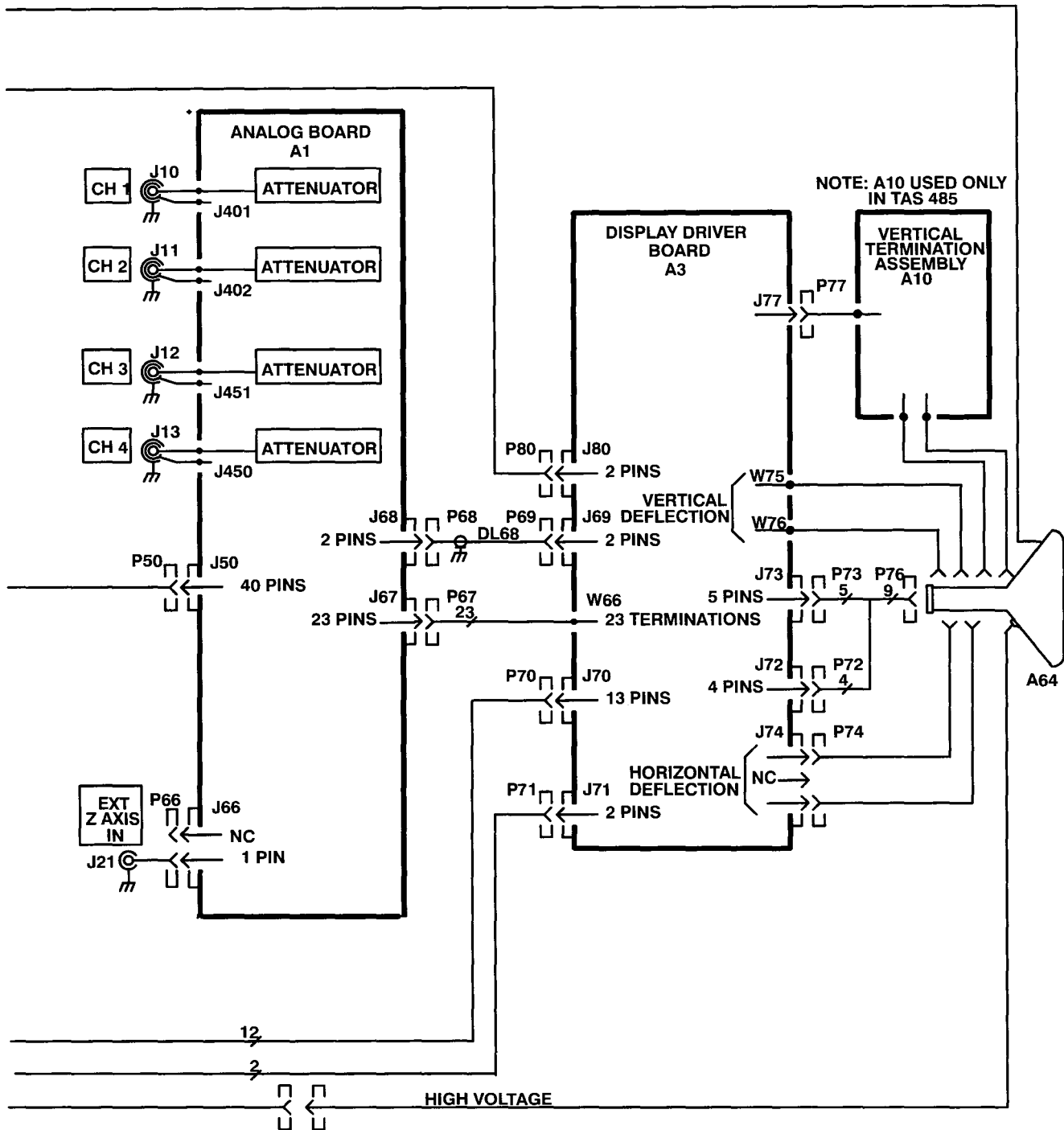
Figure 3-1: Block Diagram (Cont.)
