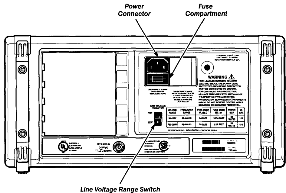
Figure 2-1: Rear Panel
