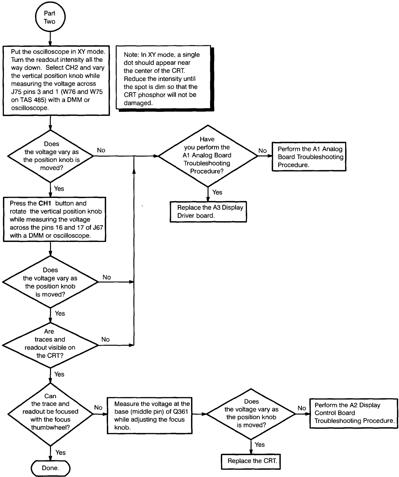
Figure 6-23: A3 Display Driver Board Troubleshooting Procedure (Cont.)
